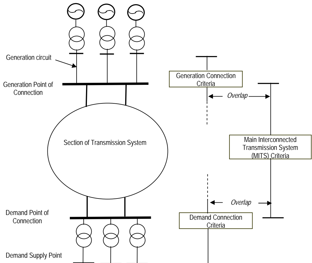
Figure: 1.1 Transmission System connected to generation and distribution sites
